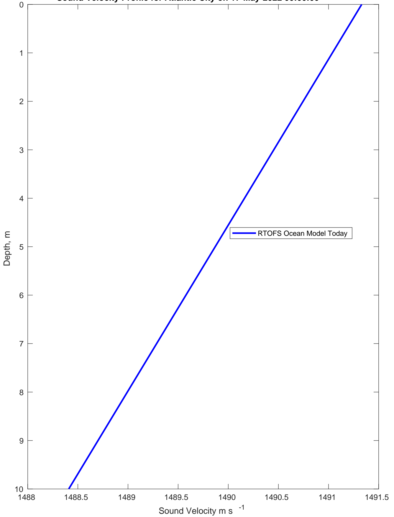
Sound Velocity Profile for Atlantic City on 17-May-2022 00:00:00
